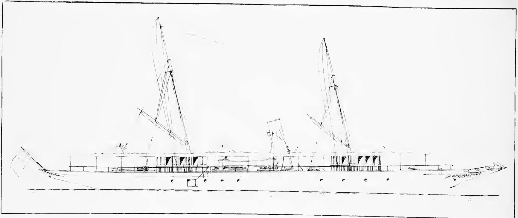
SHEAR PLAN OF THE STEAM YACHT FREE LANCE.—Built by Lewis Nixon, Elizabethport, N. J., from Designs of A. Cary Smith.
